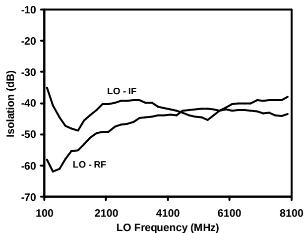
Figure 7. LO Isolation.
