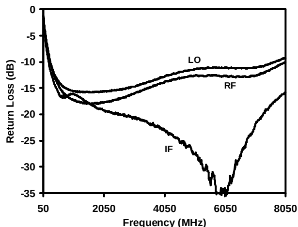
Figure 9. Return Loss.
